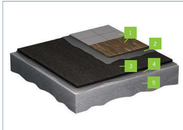
Regupol® Sonus HS 3 mm, 5 mm is a high quality full rubber and 100 % recycled impact sound underlayment.
