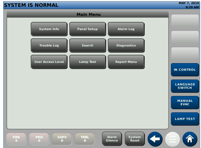
Figure 6: Main Menu
