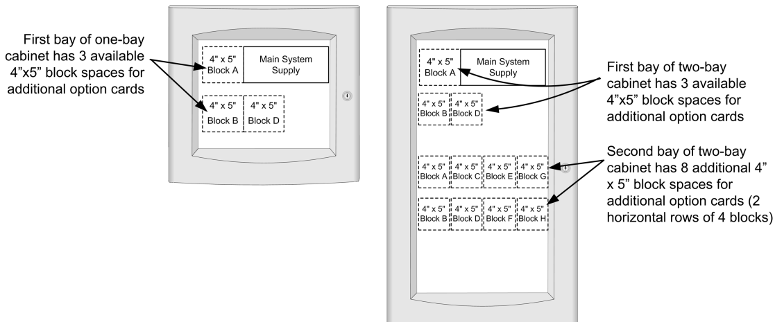
Figure 13: Loading reference
